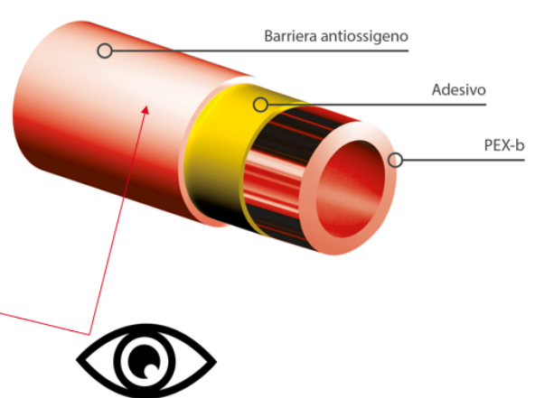
Old version 3 layer – external barrier
