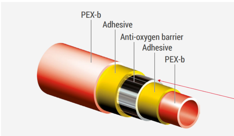
New version 5 layer – intermediate barrier
